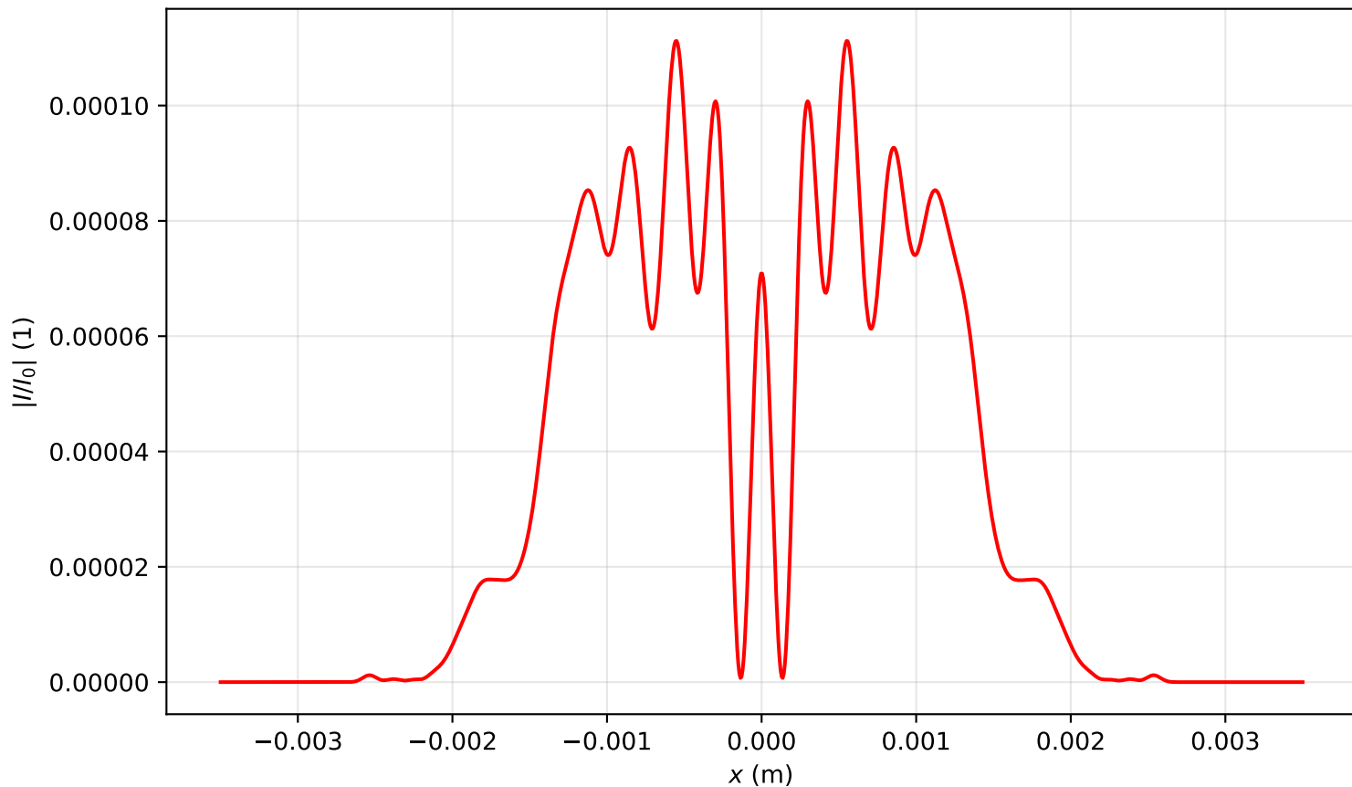
Intensity profile I(x, y = 0, z = 1.194)/I_0 , P_{in}=9.0P_{cr} , artificial time
